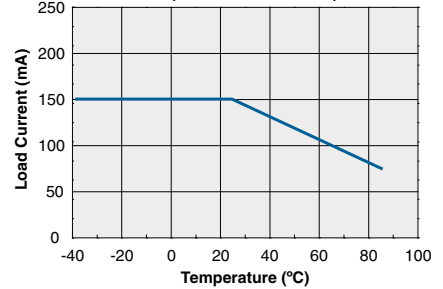
Load Current vs. Load Temperature (Form-A: I_F=5\text{mA} , Form-B: I_F=0\text{mA} )
