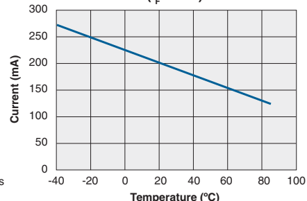
Typical Current Limiting vs. Temperature ( I_F=5\text{mA} )
