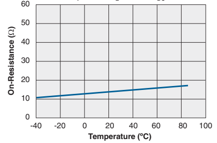
Typical On-Resistance vs. Temperature ( I_F=5\text{mA}, I_L=170\text{mA}_{DC} )
