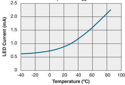
Typical I_F for Switch Operation vs. Temperature ( I_L=170\text{mA}_{DC} )
