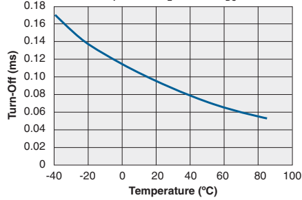
Typical Turn-Off vs. Temperature ( I_F=5\text{mA}, I_L=170\text{mA}_{DC} )
