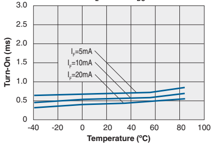
Typical Turn-On vs. Temperature ( I_L=170\text{mA}_{DC} )
