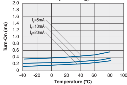
Typical Turn-On vs. Temperature ( I_L=120\text{mA}_{DC} )
