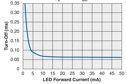
Typical Turn-Off vs. LED Forward Current ( I_L=120\text{mA}_{DC} )
