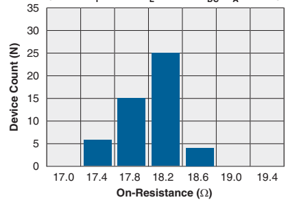
Typical On-Resistance Distribution (N=50, I_F=5\text{mA} , I_L=120\text{mA}_{DC} , T_A=25^\circ\text{C} )
