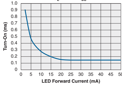
Typical Turn-On vs. LED Forward Current ( I_L=120\text{mA}_{DC} )
