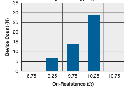
Typical On-Resistance Distribution (N=50, I_L=120mA_{DC} , T_A=25^\circ C )
