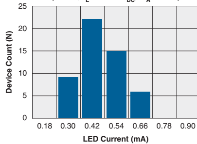
Typical I_F for Switch Dropout (N=50, I_L=120mA_{DC} , T_A=25^\circ C )
