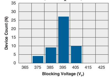
Typical Blocking Voltage Distribution (N=50, T_A=25^\circ C )
