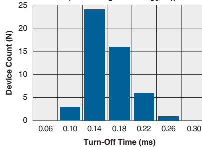
Typical Turn-Off Time (N=50, I_F=2mA , I_L=120mA_{DC} , T_A=25^\circ C )
