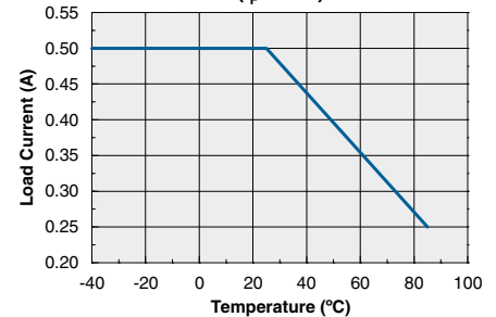
Maximum Load Current vs. Temperature ( I_F=5mA )
