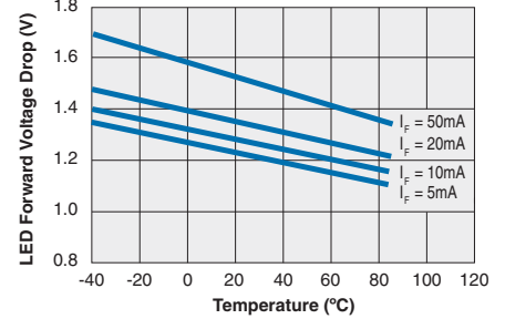
Typical LED Forward Voltage Drop vs. Temperature
