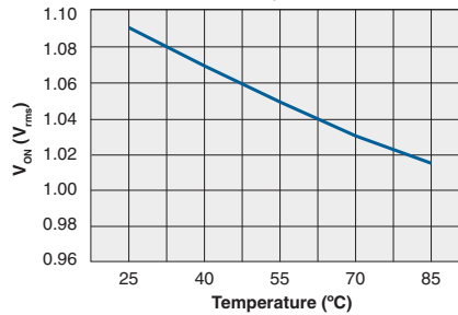
Typical Output V_{ON} vs. Temperature
