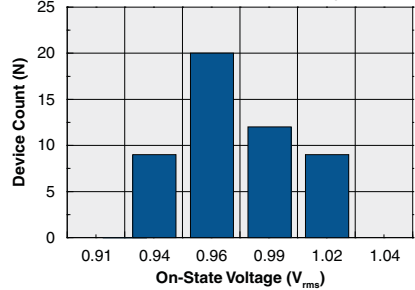
Typical On-State Voltage Distribution ( T_A=25^\circ\text{C} , I_L=500\text{mA}_{\text{rms}} )
