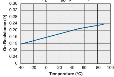
Typical On-Resistance vs. Temperature ( I_L=1.0\text{A}_{DC}, I_F=10\text{mA} )
