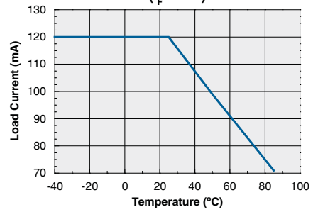
Typical Load Current vs. Temperature ( I_F=2mA )
