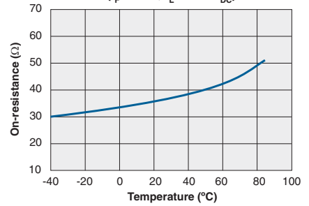
Typical On-Resistance vs. Temperature ( I_F=2mA, I_L=50mA_{DC} )
