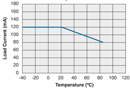
Typical Load Current vs. Temperature ( I_F=0\text{mA} )
