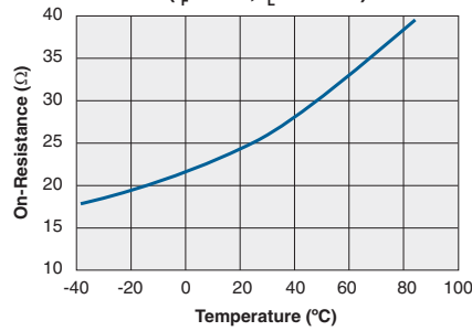
Typical On-Resistance vs. Temperature ( I_F=0\text{mA} , I_L=120\text{mA} )
