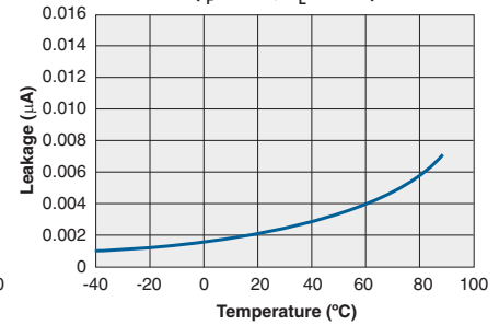
Typical Leakage vs. Temperature Measured Across Pins 3&4 ( I_F=2\text{mA} , V_L=350\text{V} )
