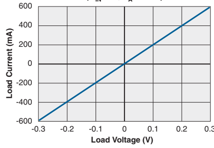
Typical Load Current vs. Load Voltage ( V_{IN}=5V, T_A=25°C )
