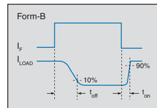
Switching Characteristics of Normally Closed Devices
