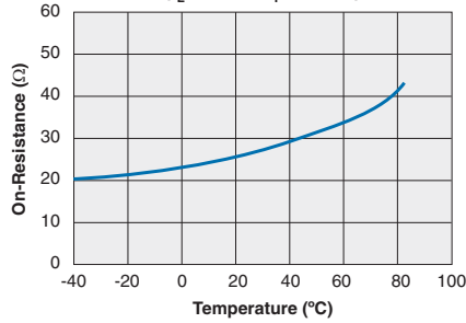
Typical On-Resistance vs. Temperature ( I_L=80mA, I_F=10mA )
