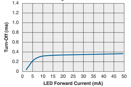
Typical Turn-Off vs. LED Forward Current ( I_L=120mA )
