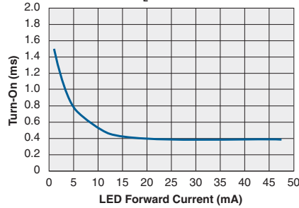
Typical Turn-On vs. LED Forward Current ( I_L=120mA )
