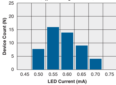
Typical I F for Switch Operation ( T_A=25^\circ\text{C} , I_L=120\text{mA} )
