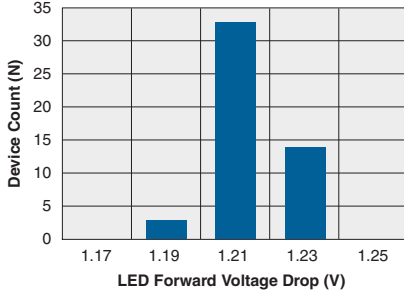
CPC1002N Typical LED Forward Voltage Drop ( T_A=25^\circ\text{C} , I_F=5\text{mA} )
